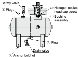
Drain valve: VBAT-V1
