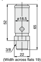
Safety valve: VBAT-R, VBAT-S
